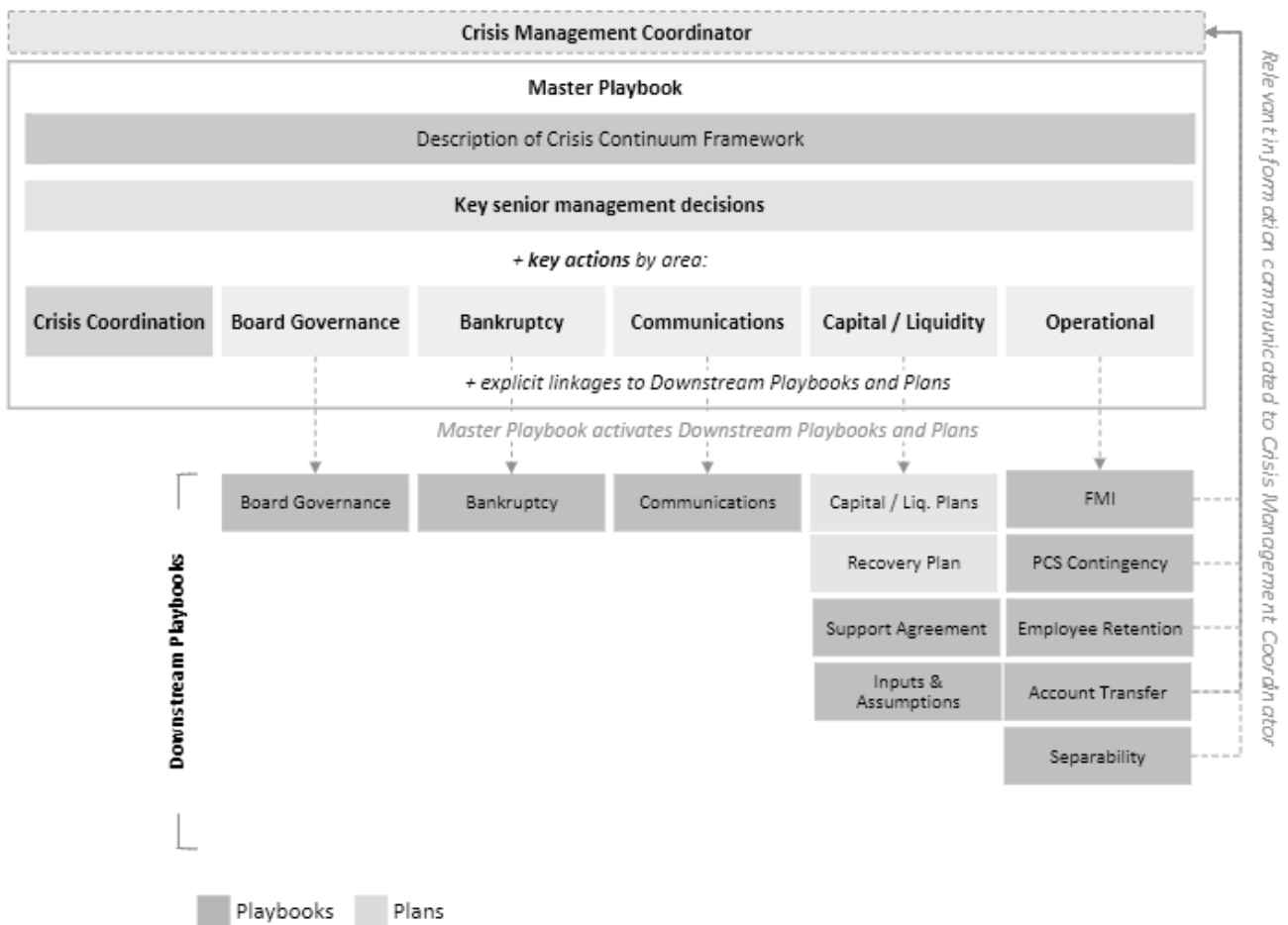
Figure 4.3-3: Playbook Architecture
