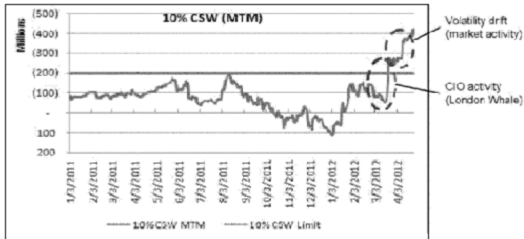
CIO Mark-to-Market CSW10% Breaches January 2011-April 2012
