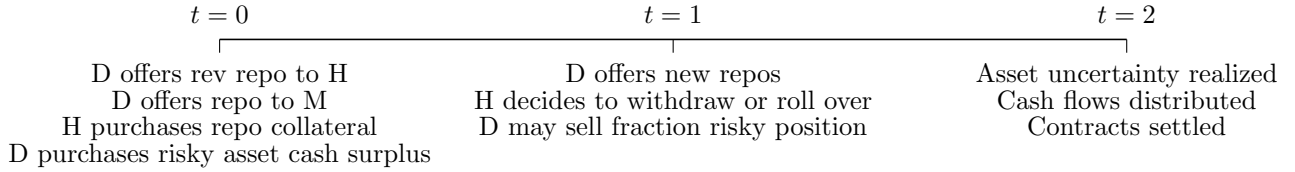
Figure 3: Model Timeline
