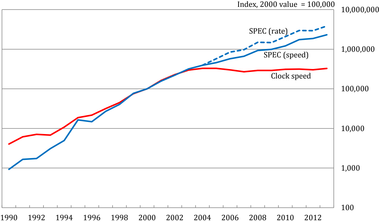
Figure 1: Desktop MPU Performance Measures
