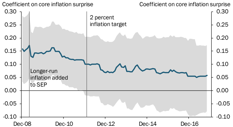
Chart 1: Coefficient on core inflation surprises over time
