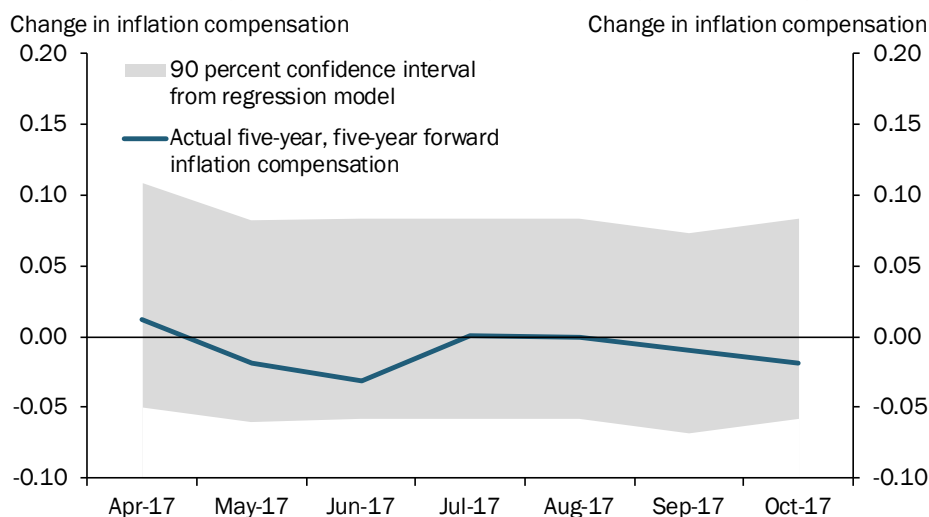
Chart 2: Actual and predicted inflation compensation response to CPI reports
