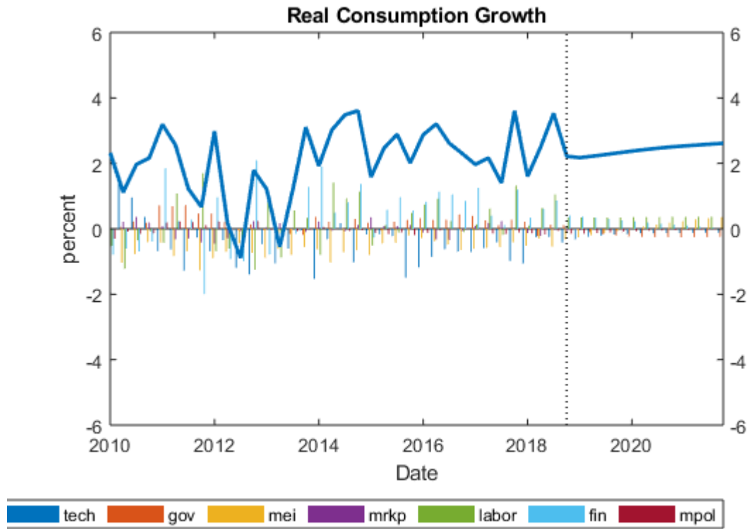
Figure 2d Shock Decompositions
