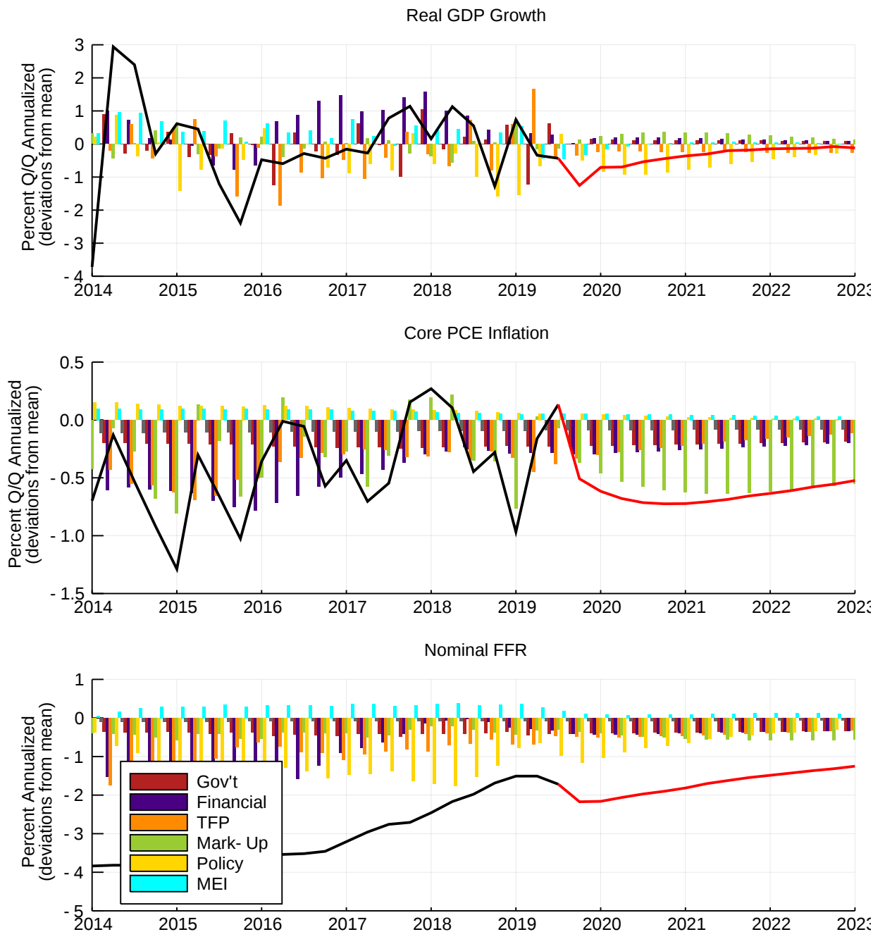
Figure 3: Shock Decomposition
