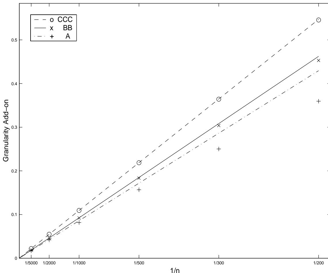
Figure 1: Granularity Add-on as Linear Function of 1/n
