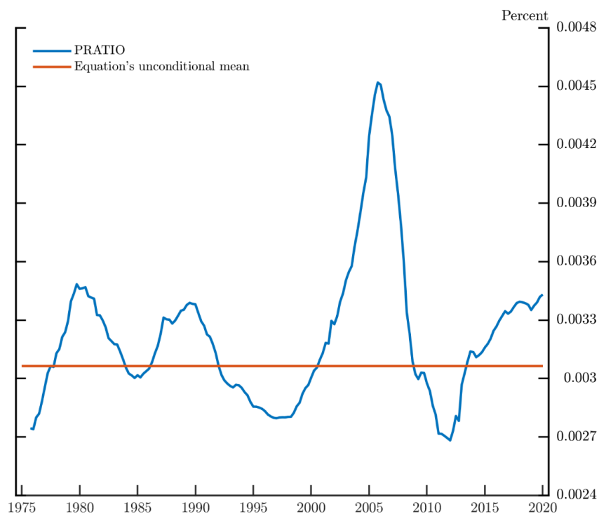
Figure I1 – PRATIO and equation’s unconditional mean
