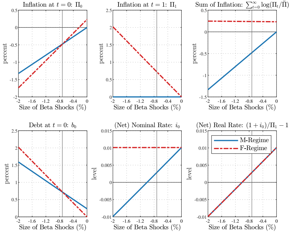
Appendix Figure B.2: Variable Responses by Different Size of Beta Shocks with \varphi = 0 (Infinite Frisch elasticity)
